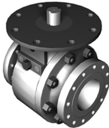
Figure 1 Typical C-Series Floating Ball Valve covered in this FMEDA,
